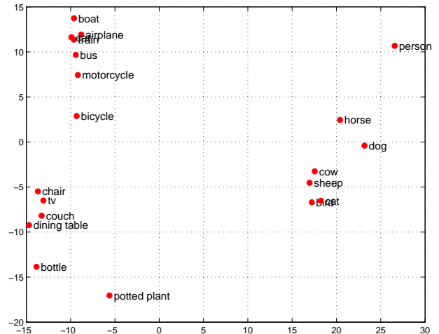
Figure 4. Visualizing 20 PASCAL VOC object classes in the semantic affordance space.
